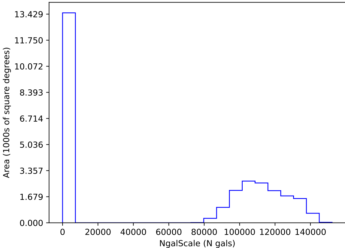
too_elab_heavy_r64_d3_gz_v3.4_10yrs i: NgalScale
