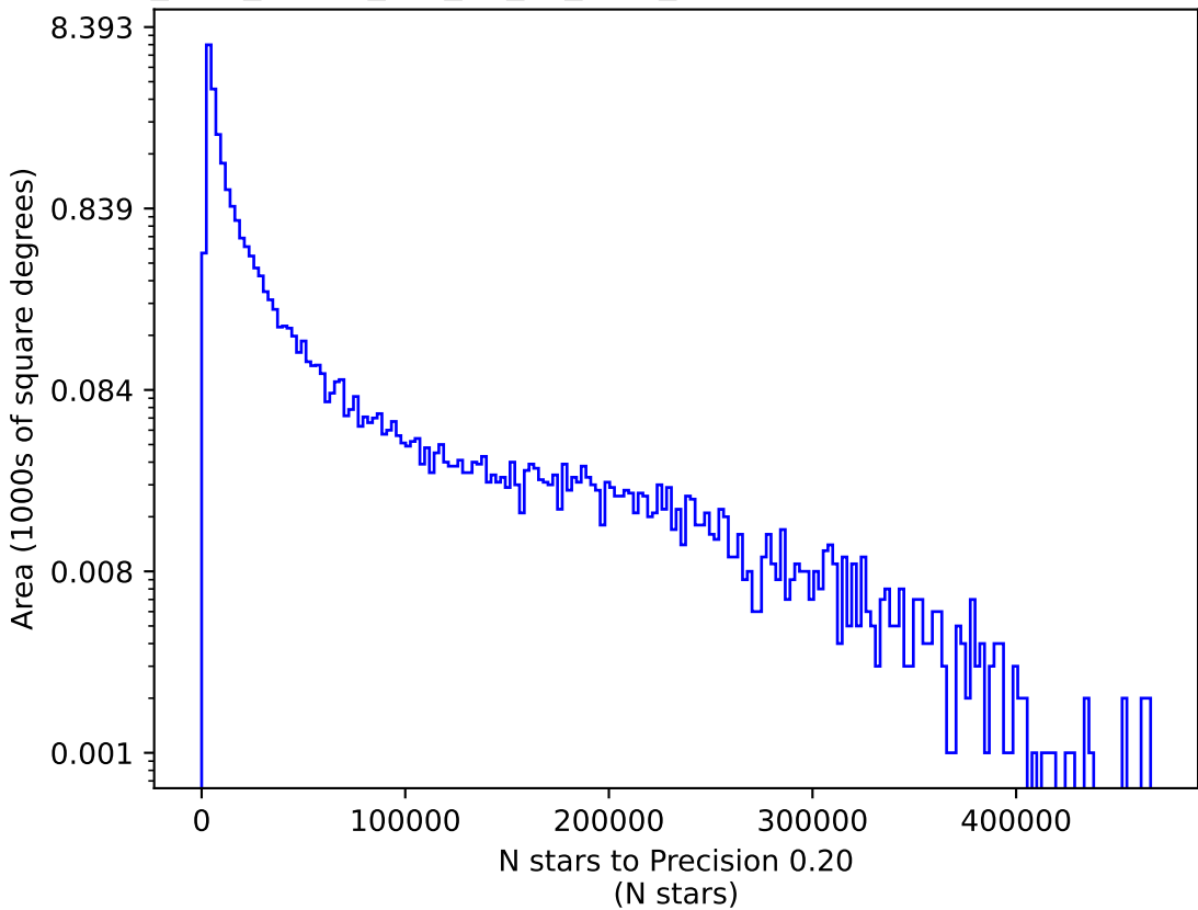
too_elab_heavy_r64_d3_gz_v3.4_10yrs u: N stars to Precision 0.20
