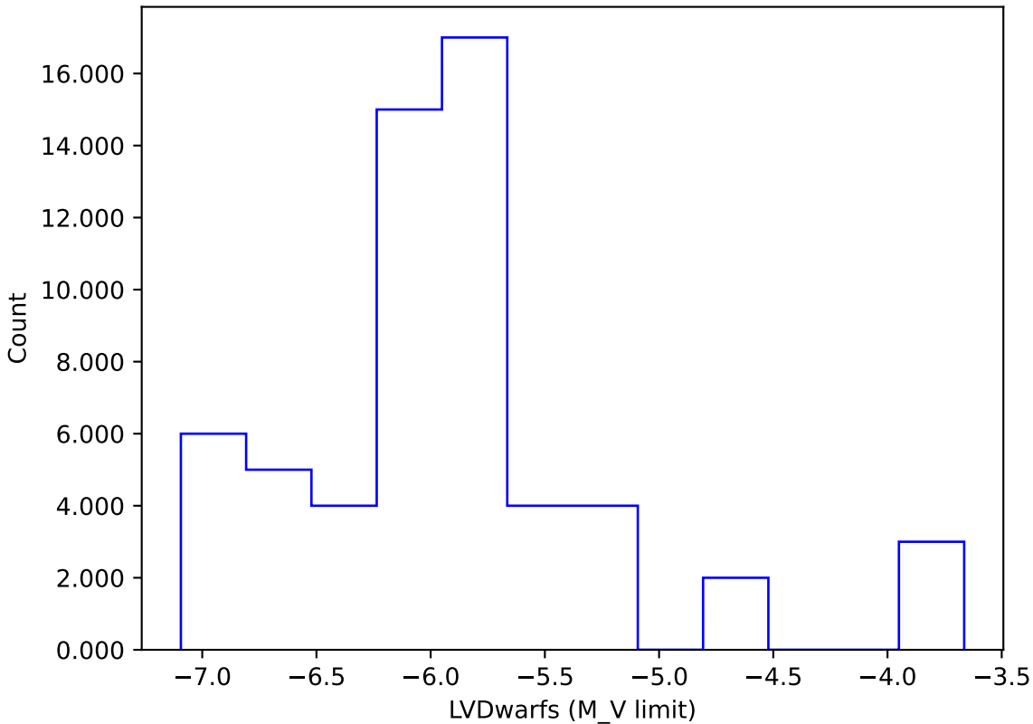
too_elab_heavy_r64_d3_gz_v3.4_10yrs gi: LVDwarfs
