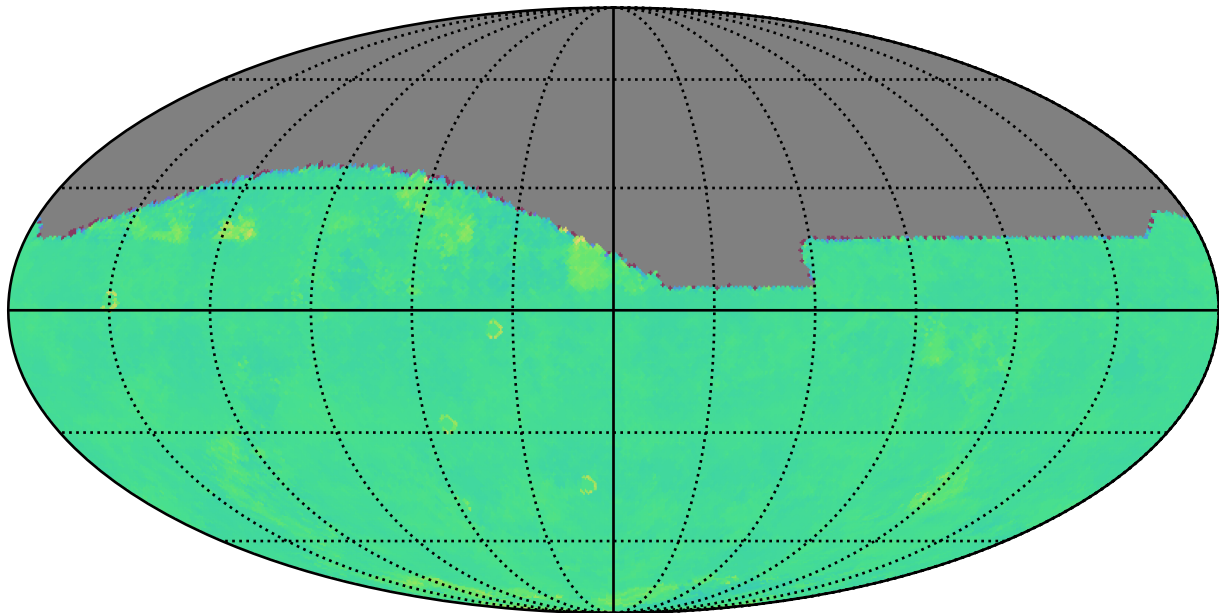
too_elab_heavy_r64_d3_gz_v3.4_10yrs z: Kuiper rotTelPos
