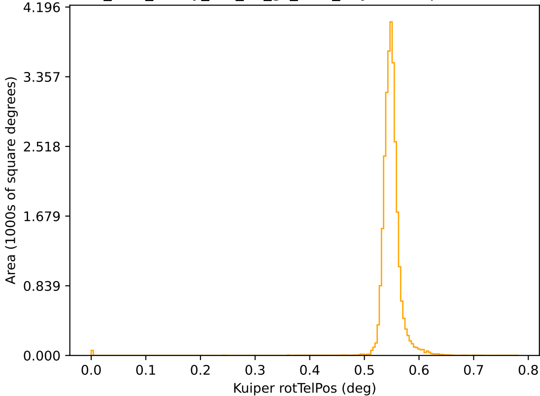
too_elab_heavy_r64_d3_gz_v3.4_10yrs r: Kuiper rotTelPos
