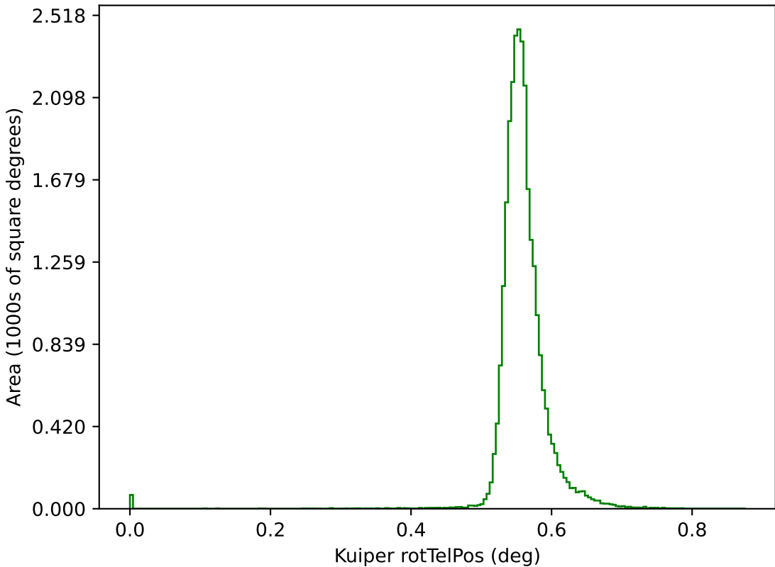
too_elab_heavy_r64_d3_gz_v3.4_10yrs g: Kuiper rotTelPos
