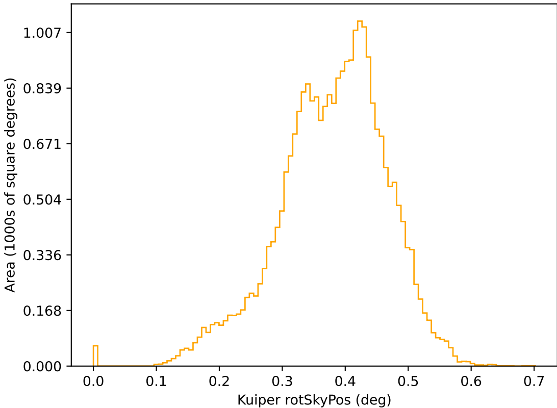
too_elab_heavy_r64_d3_gz_v3.4_10yrs r: Kuiper rotSkyPos
