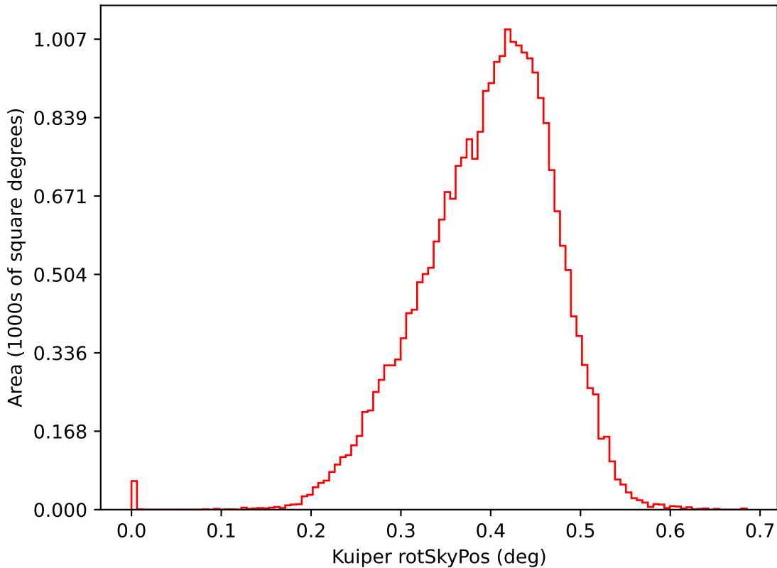
too_elab_heavy_r64_d3_gz_v3.4_10yrs i: Kuiper rotSkyPos
