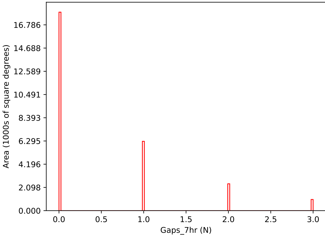
too_elab_heavy_r64_d3_gz_v3.4_10yrs i band: Gaps_7hr
