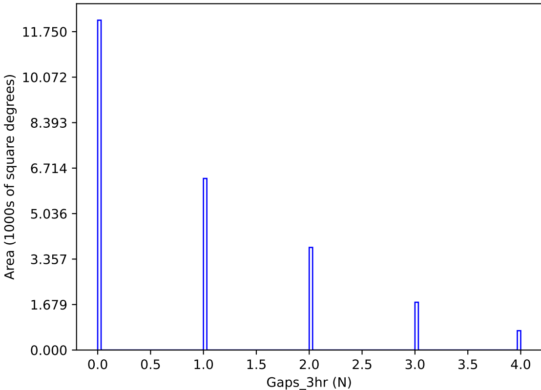
too_elab_heavy_r64_d3_gz_v3.4_10yrs y band: Gaps_3hr
