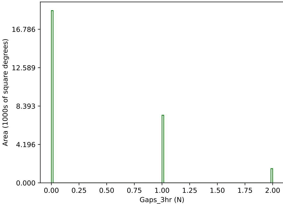
too_elab_heavy_r64_d3_gz_v3.4_10yrs g band: Gaps_3hr
