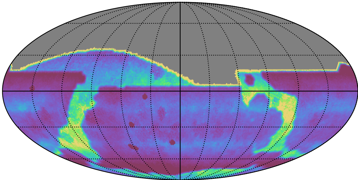
too_elab_heavy_r64_d3_gz_v3.4_10yrs : DCRprecision
