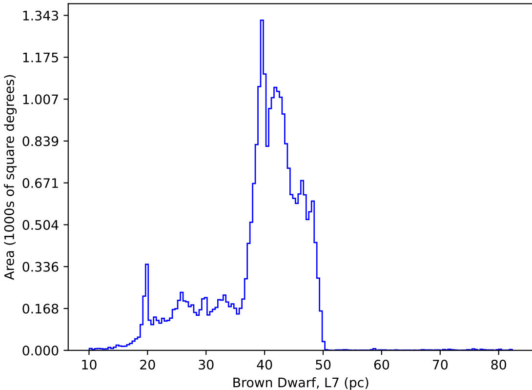
too_elab_heavy_r64_d3_gz_v3.4_10yrs : Brown Dwarf, L7
