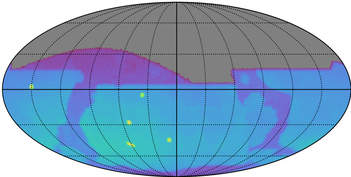
too_elab_heavy_r64_d3_gz_v3.4_10yrs : Brown Dwarf, L4
