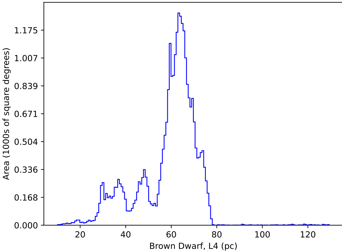
too_elab_heavy_r64_d3_gz_v3.4_10yrs : Brown Dwarf, L4
