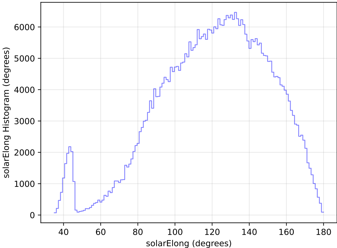
too_elab_heavy_r64_d3_gz_v3.4_10yrs WFD z band: solarElong Histogram
