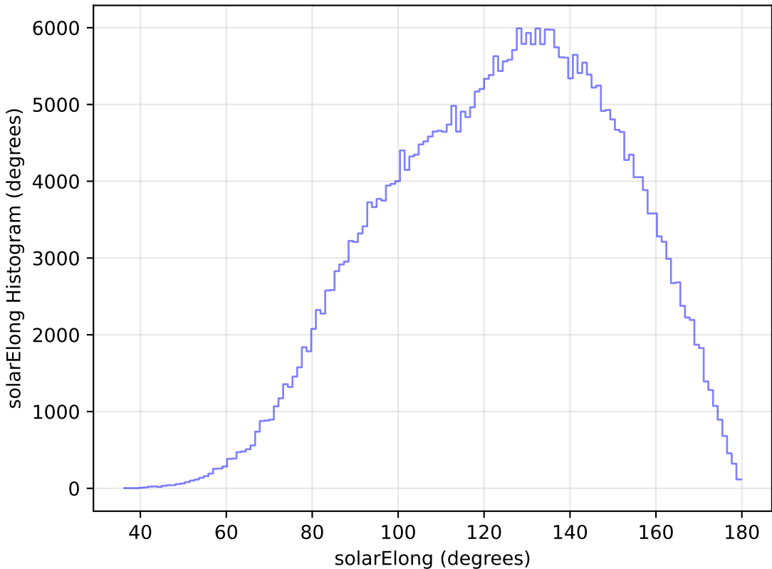
too_elab_heavy_r64_d3_gz_v3.4_10yrs WFD y band: solarElong Histogram
