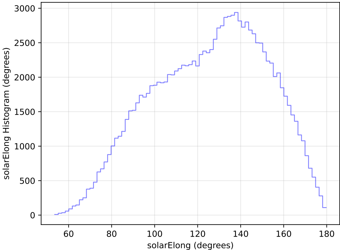
too_elab_heavy_r64_d3_gz_v3.4_10yrs WFD u band: solarElong Histogram
