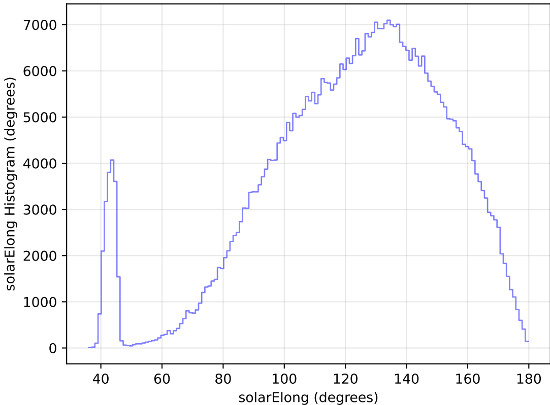
too_elab_heavy_r64_d3_gz_v3.4_10yrs WFD r band: solarElong Histogram
