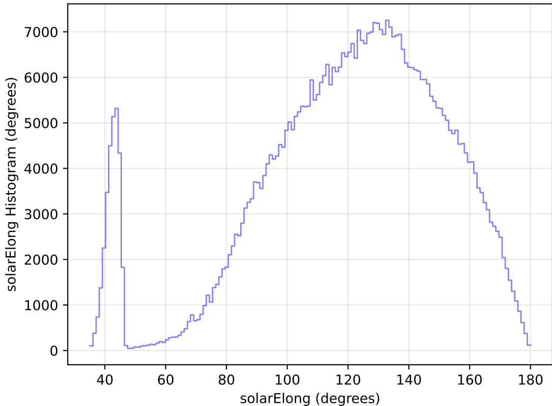
too_elab_heavy_r64_d3_gz_v3.4_10yrs WFD i band: solarElong Histogram
