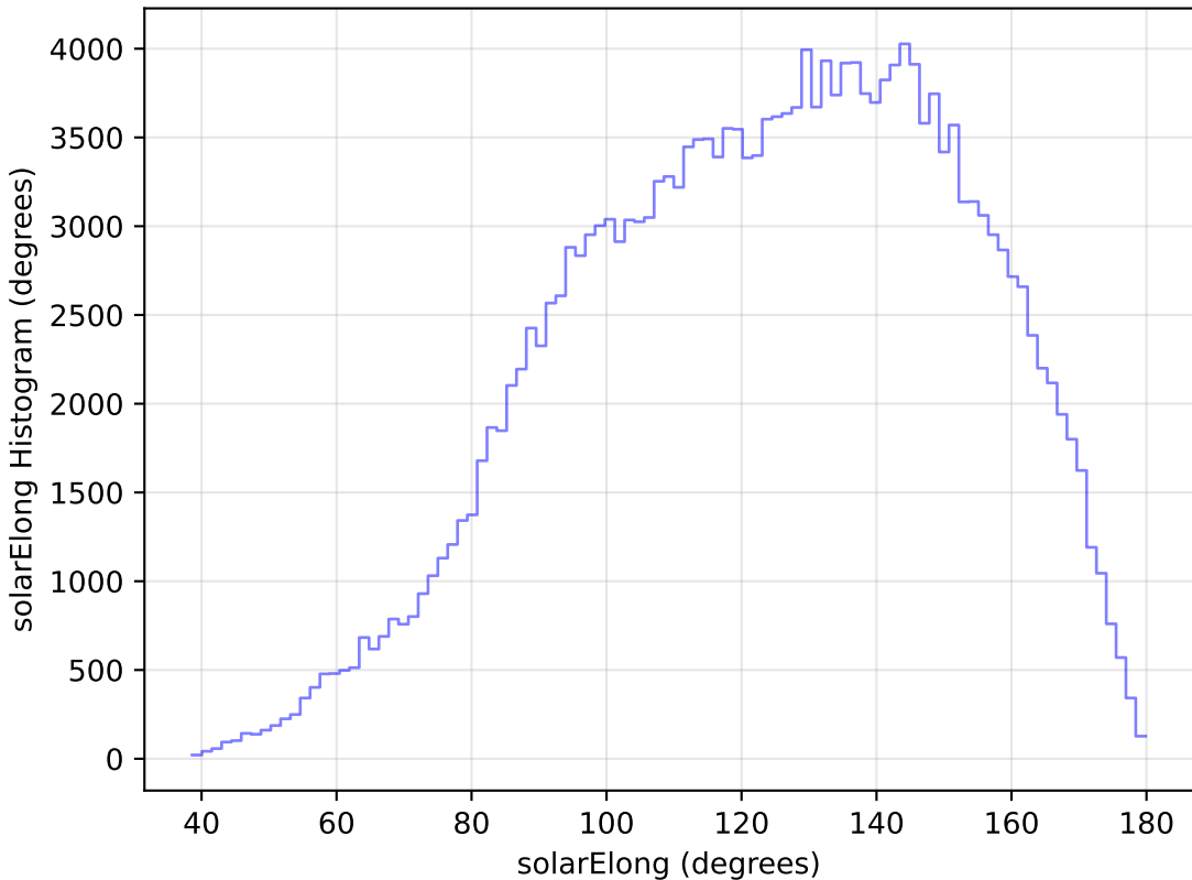
too_elab_heavy_r64_d3_gz_v3.4_10yrs WFD g band: solarElong Histogram
