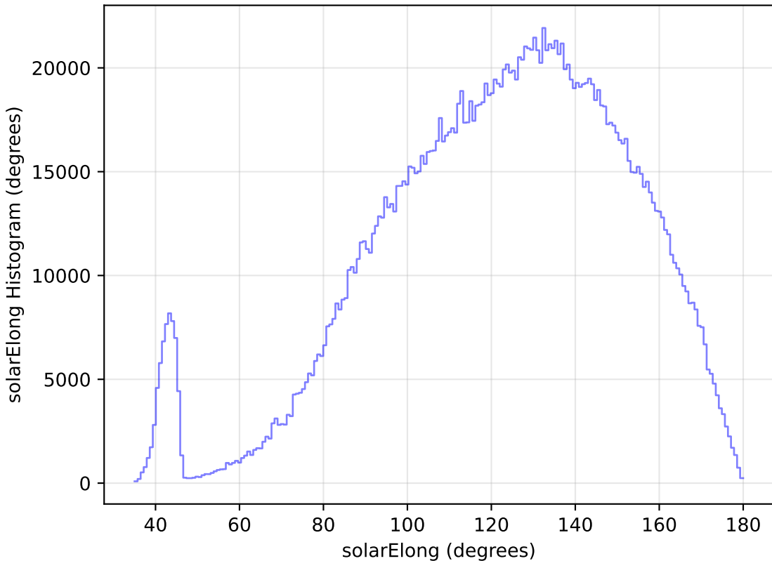
too_elab_heavy_r64_d3_gz_v3.4_10yrs WFD all bands: solarElong Histogram
