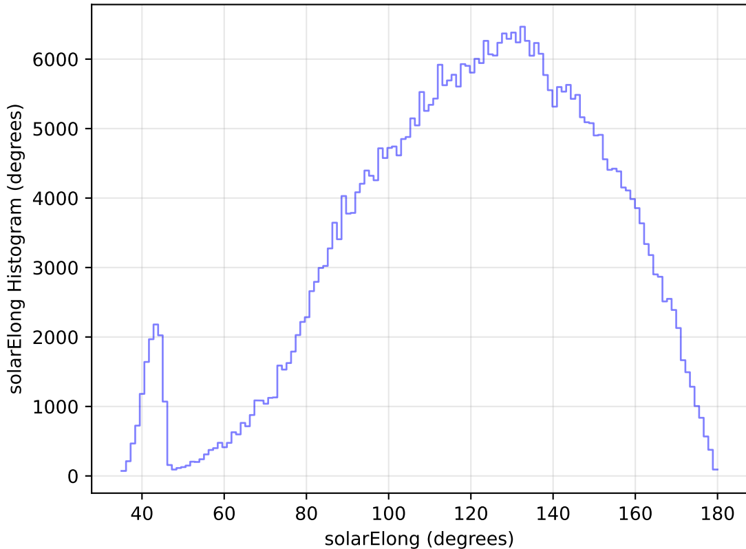
too_elab_heavy_r64_d3_gz_v3.4_10yrs All sky z band: solarElong Histogram
