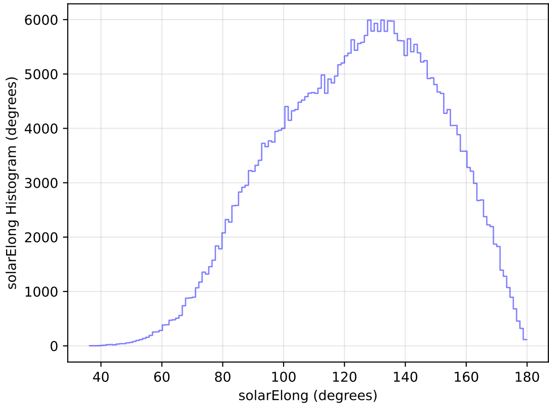
too_elab_heavy_r64_d3_gz_v3.4_10yrs All sky y band: solarElong Histogram
