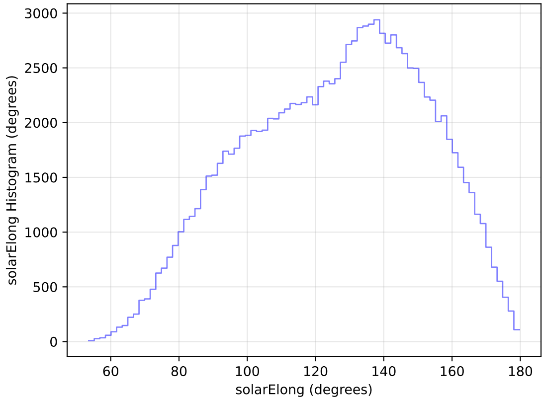
too_elab_heavy_r64_d3_gz_v3.4_10yrs All sky u band: solarElong Histogram
