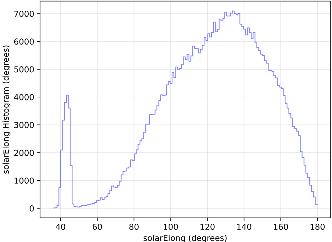
too_elab_heavy_r64_d3_gz_v3.4_10yrs All sky r band: solarElong Histogram
