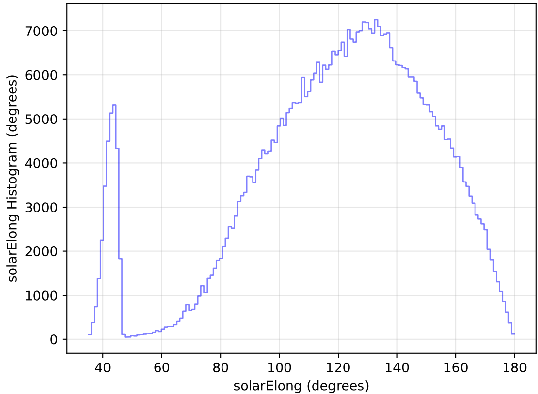
too_elab_heavy_r64_d3_gz_v3.4_10yrs All sky i band: solarElong Histogram
