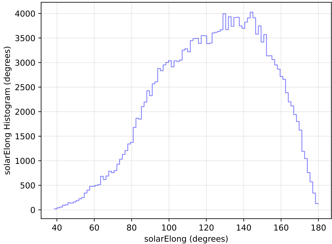
too_elab_heavy_r64_d3_gz_v3.4_10yrs All sky g band: solarElong Histogram
