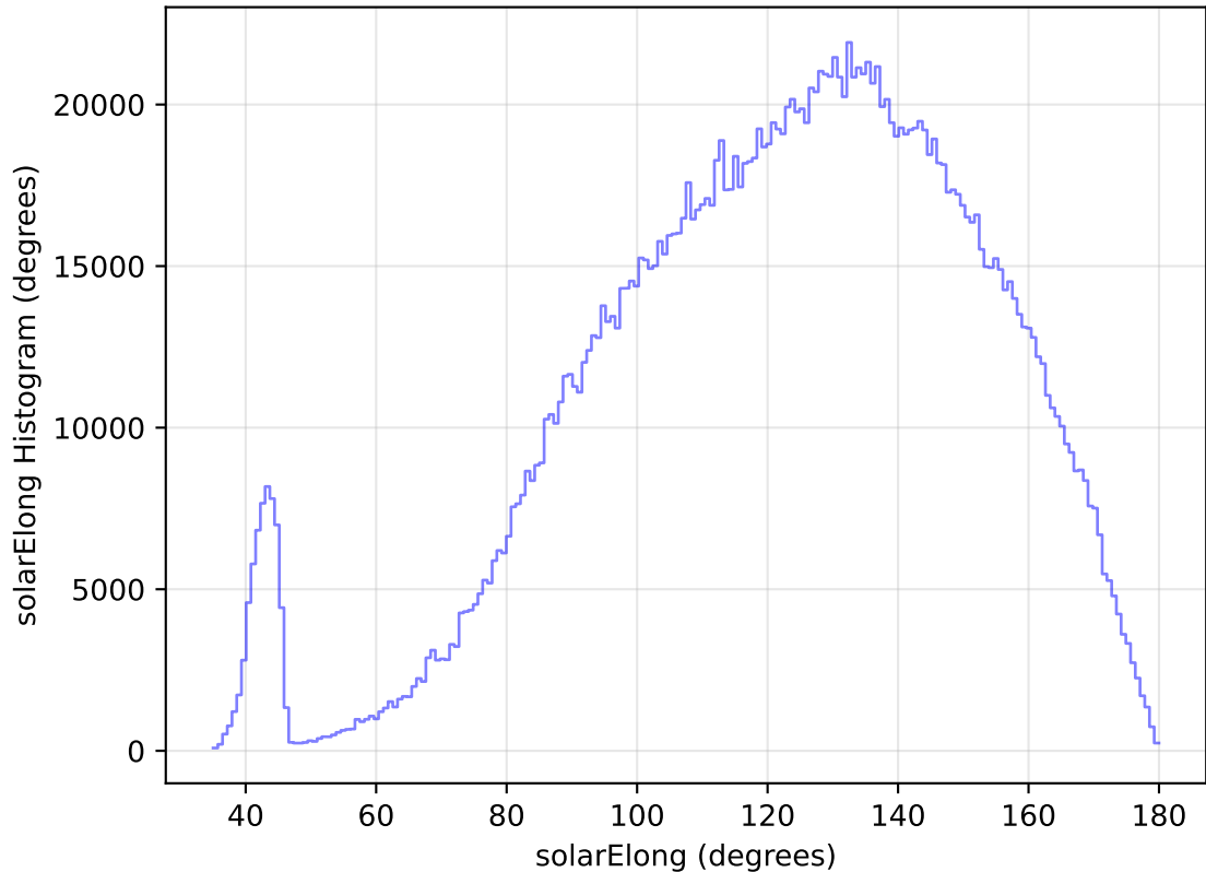
too_elab_heavy_r64_d3_gz_v3.4_10yrs All sky all bands: solarElong Histogram
