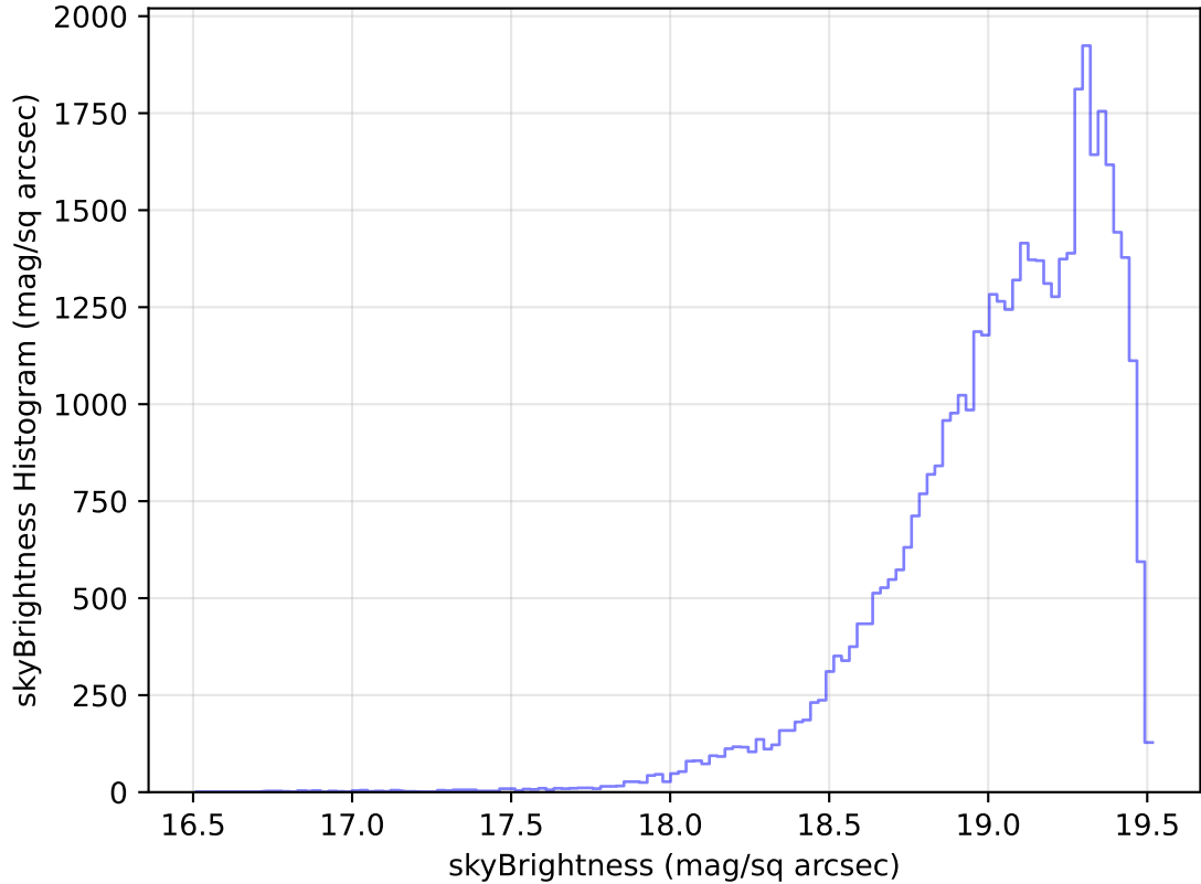
too_elab_heavy_r64_d3_gz_v3.4_10yrs Yr 1 z band: skyBrightness Histogram
