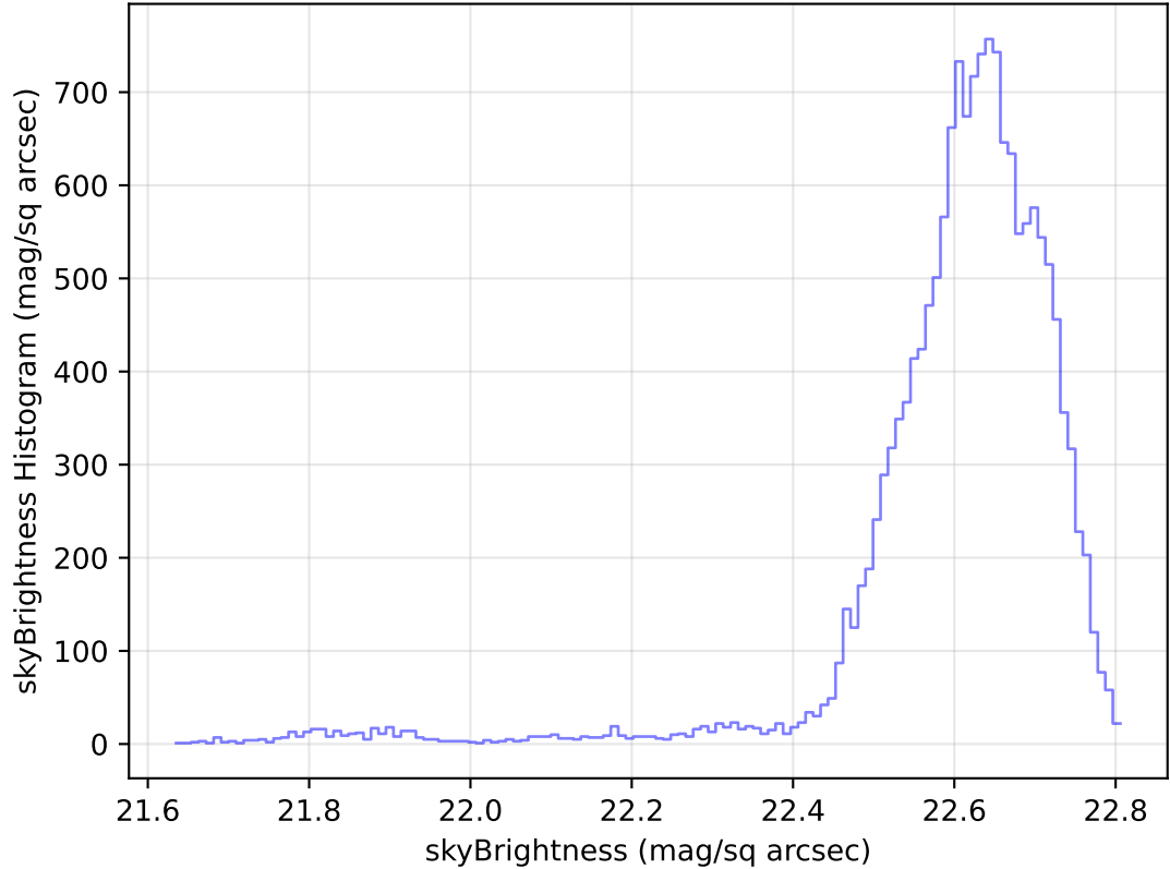
too_elab_heavy_r64_d3_gz_v3.4_10yrs Yr 1 u band: skyBrightness Histogram
