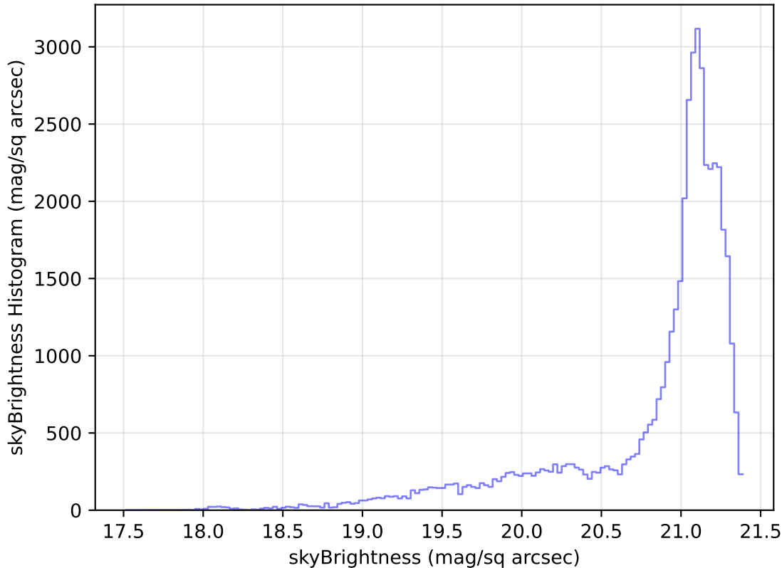
too_elab_heavy_r64_d3_gz_v3.4_10yrs Yr 1 r band: skyBrightness Histogram
