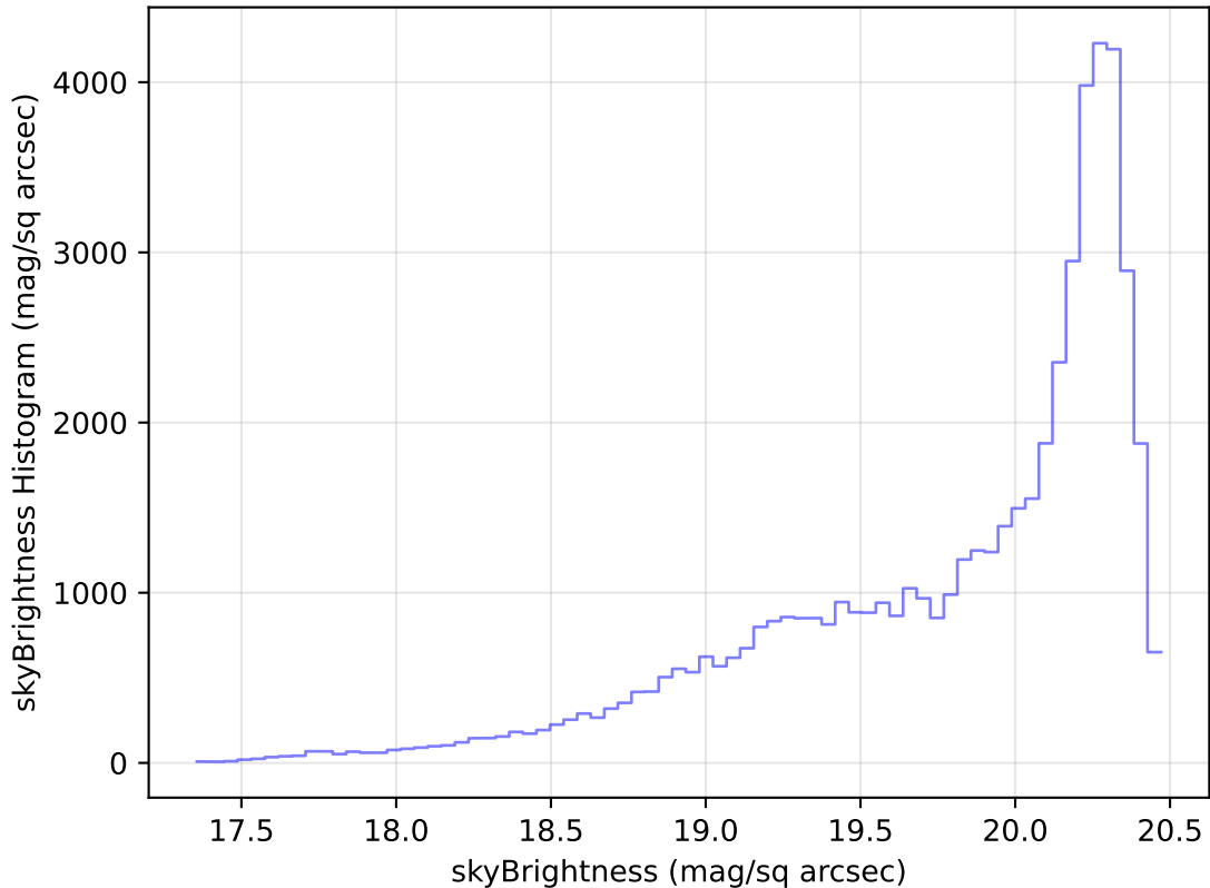
too_elab_heavy_r64_d3_gz_v3.4_10yrs Yr 1 i band: skyBrightness Histogram
