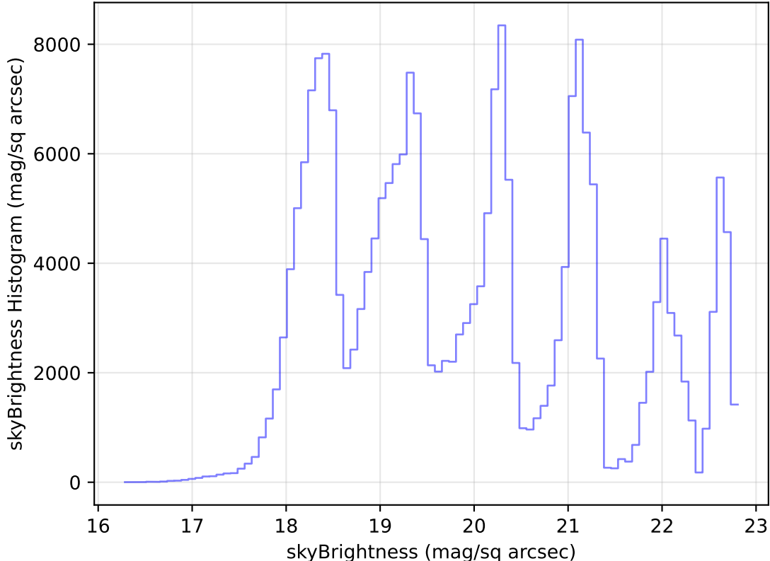
too_elab_heavy_r64_d3_gz_v3.4_10yrs Yr 1 all bands: skyBrightness Histogram
