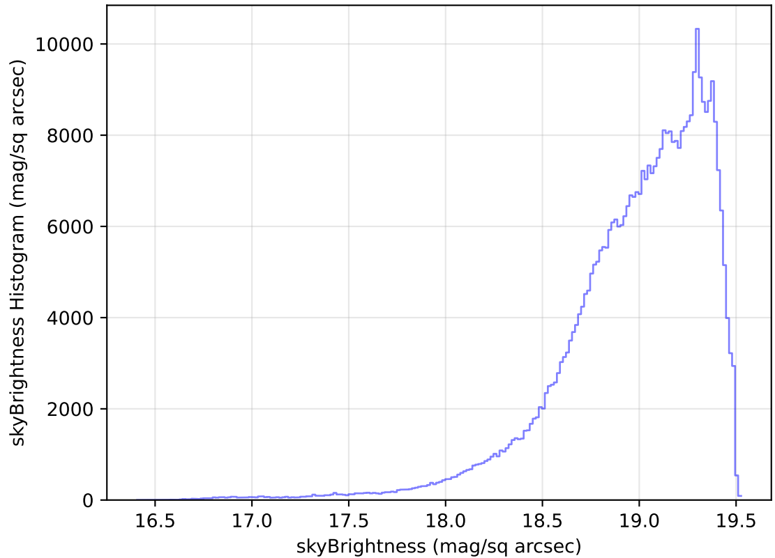
too_elab_heavy_r64_d3_gz_v3.4_10yrs WFD z band: skyBrightness Histogram
