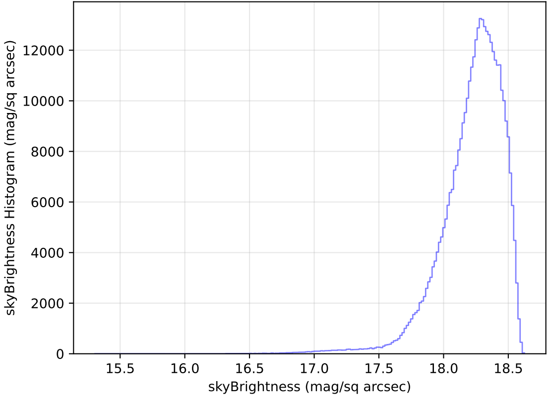
too_elab_heavy_r64_d3_gz_v3.4_10yrs WFD y band: skyBrightness Histogram
