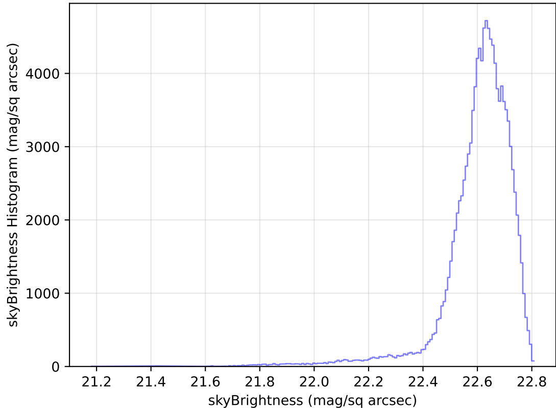
too_elab_heavy_r64_d3_gz_v3.4_10yrs WFD u band: skyBrightness Histogram
