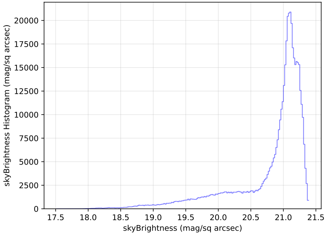
too_elab_heavy_r64_d3_gz_v3.4_10yrs WFD r band: skyBrightness Histogram
