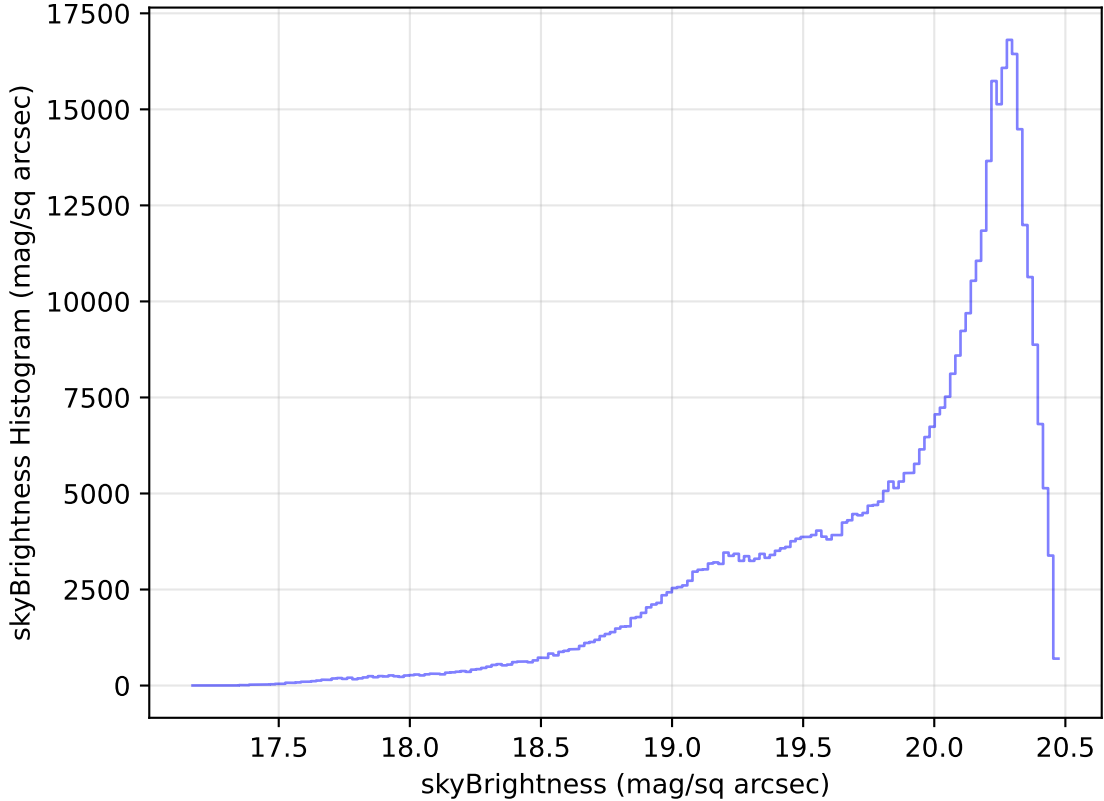
too_elab_heavy_r64_d3_gz_v3.4_10yrs WFD i band: skyBrightness Histogram
