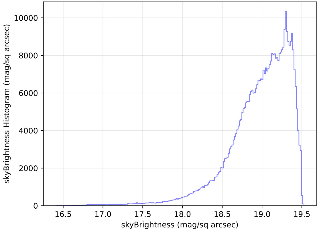
too_elab_heavy_r64_d3_gz_v3.4_10yrs All sky z band: skyBrightness Histogram
