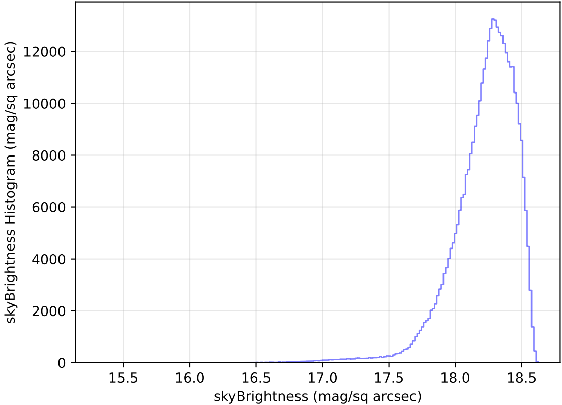
too_elab_heavy_r64_d3_gz_v3.4_10yrs All sky y band: skyBrightness Histogram
