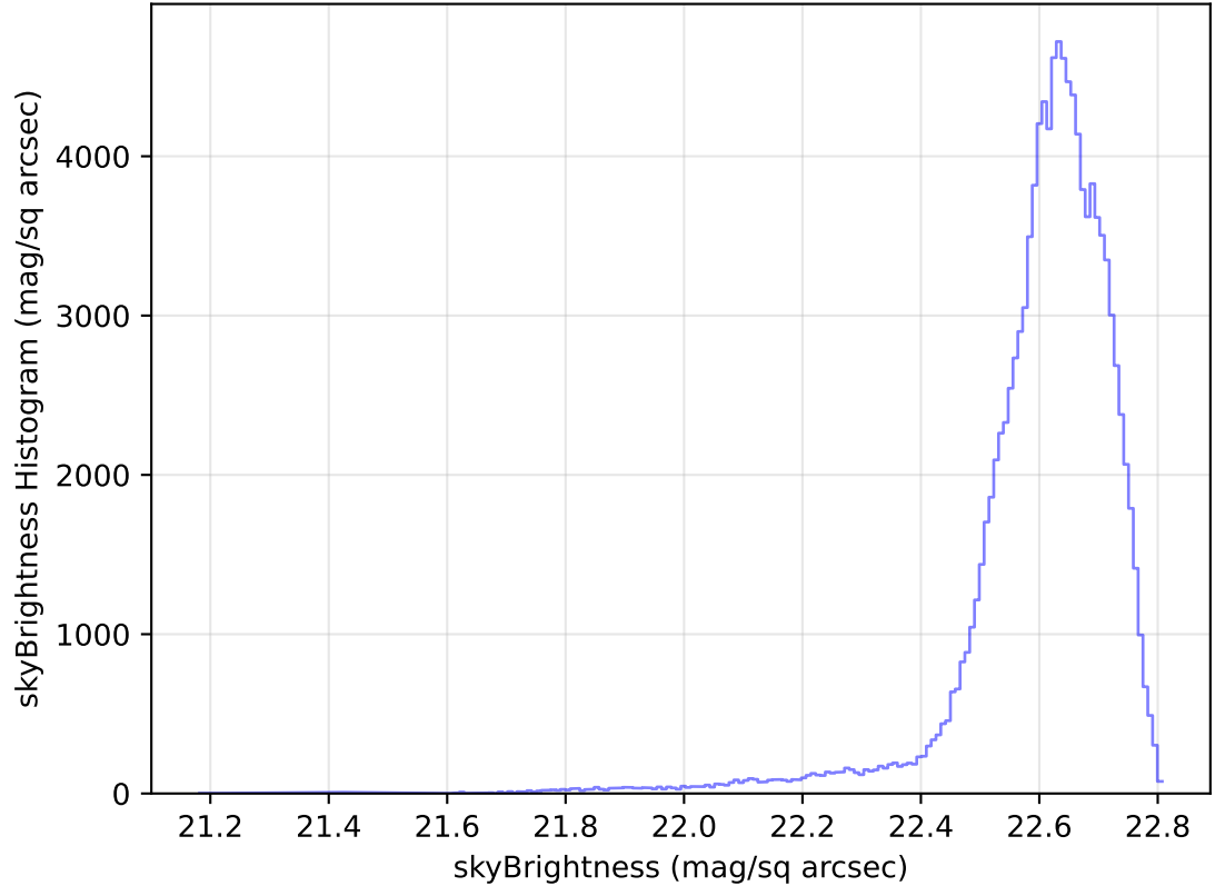
too_elab_heavy_r64_d3_gz_v3.4_10yrs All sky u band: skyBrightness Histogram
