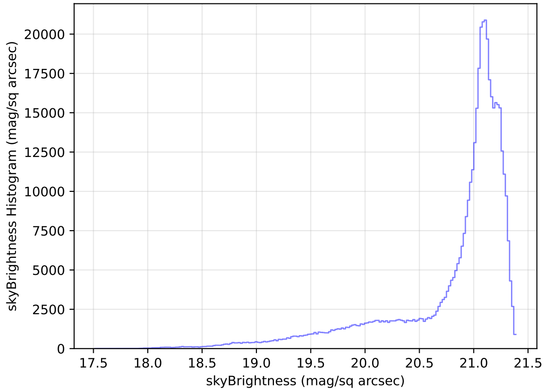
too_elab_heavy_r64_d3_gz_v3.4_10yrs All sky r band: skyBrightness Histogram
