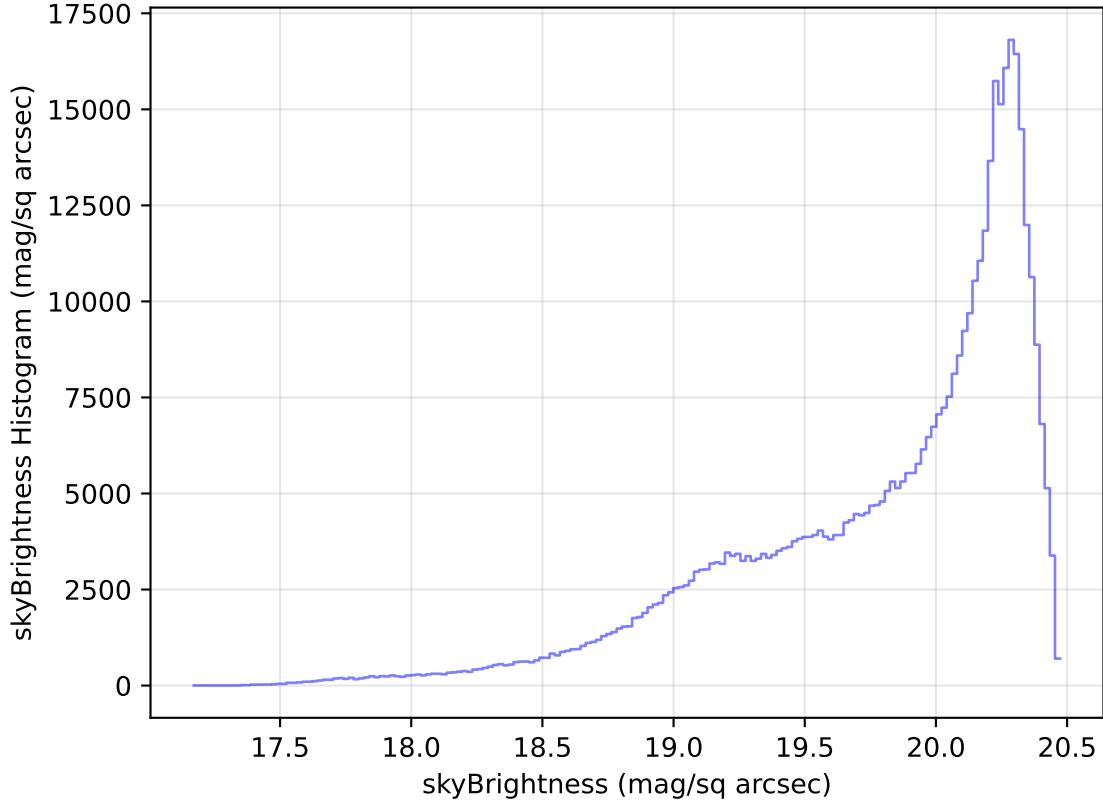
too_elab_heavy_r64_d3_gz_v3.4_10yrs All sky i band: skyBrightness Histogram
