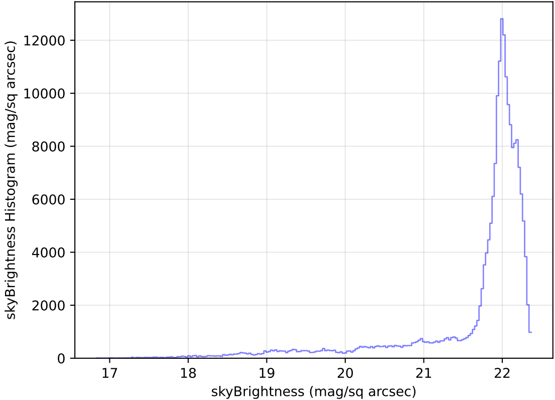
too_elab_heavy_r64_d3_gz_v3.4_10yrs All sky g band: skyBrightness Histogram
