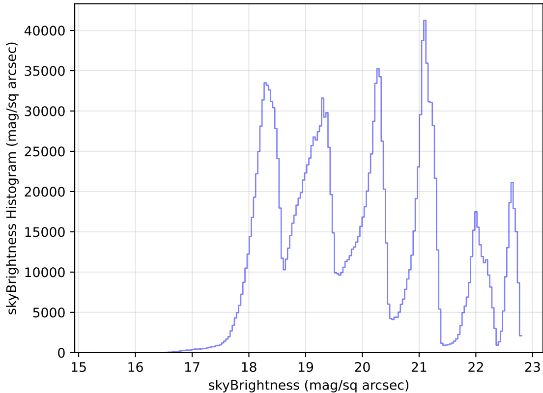
too_elab_heavy_r64_d3_gz_v3.4_10yrs All sky all bands: skyBrightness Histogram
