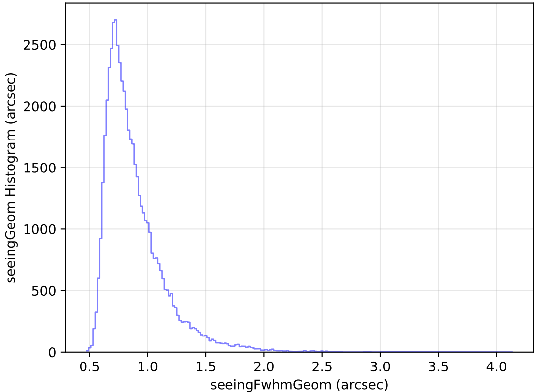
too_elab_heavy_r64_d3_gz_v3.4_10yrs Yr 1 i band: seeingGeom Histogram
