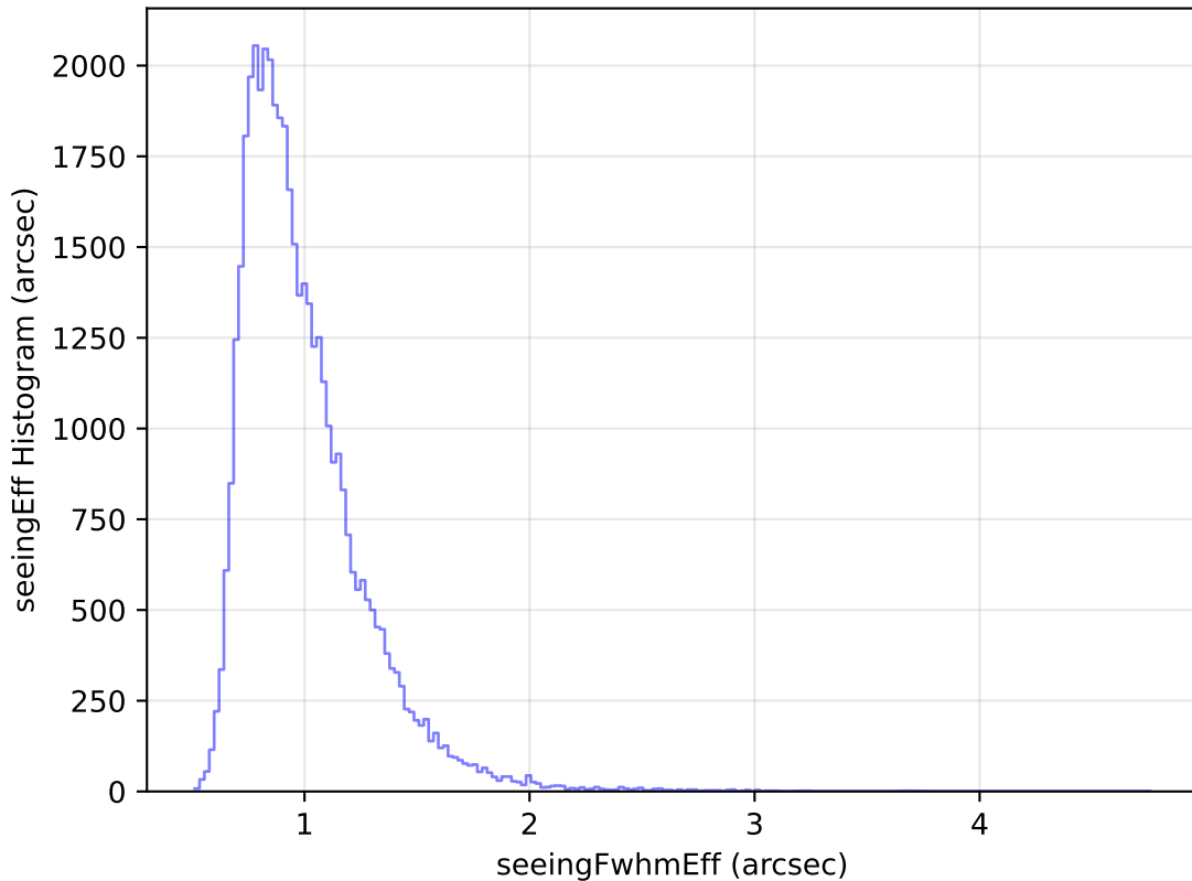
too_elab_heavy_r64_d3_gz_v3.4_10yrs Yr 1 z band: seeingEff Histogram
