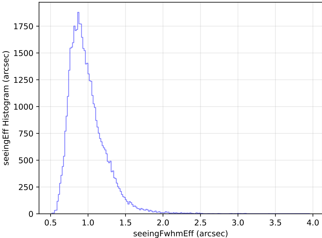
too_elab_heavy_r64_d3_gz_v3.4_10yrs Yr 1 y band: seeingEff Histogram
