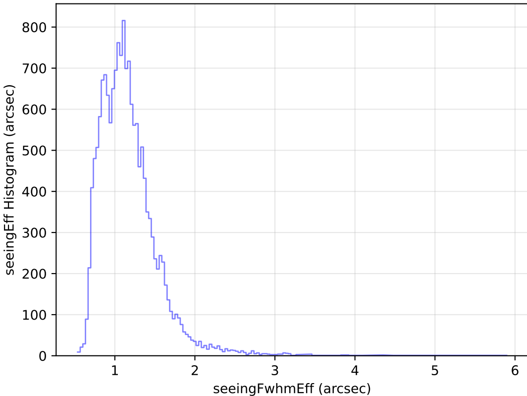
too_elab_heavy_r64_d3_gz_v3.4_10yrs Yr 1 u band: seeingEff Histogram
